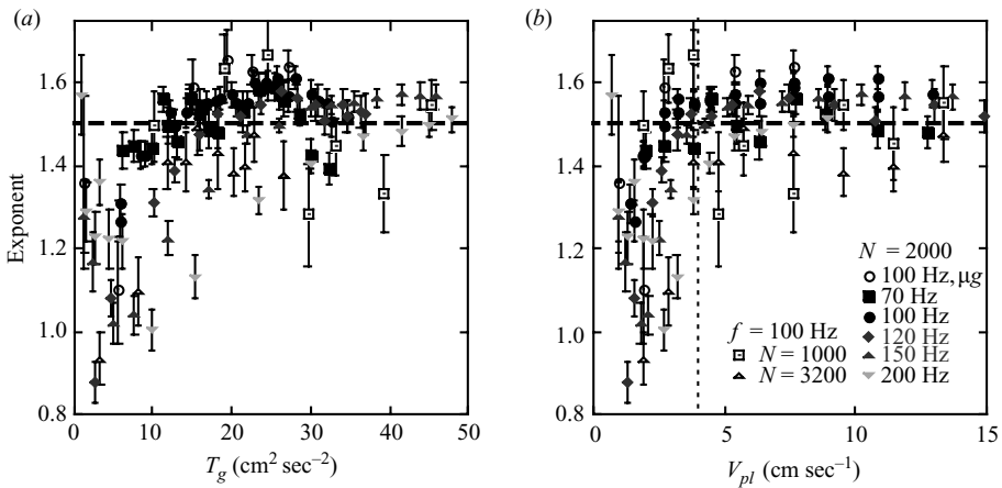
FIGURE 6. Dependence of the exponent \beta for the VDF on T_g (a) and v_{pl} (b). Dotted lines are to guide the eyes, and their value is 1.5 . The legends are common for plots in both (a) and (b).
