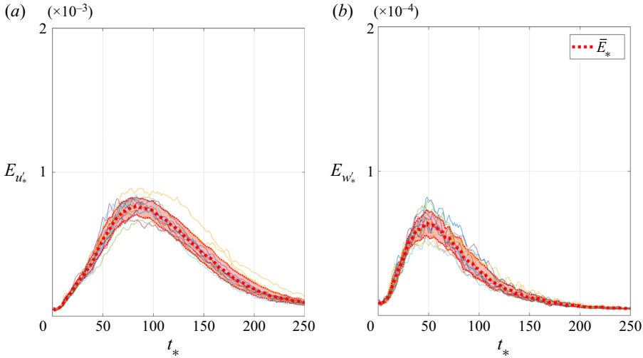
Figure 4. Energy evolution of (a) streamwise u'_* and (b) spanwise w'_* velocity fluctuations for Re = 380 and A = 82 . The red dashed curve represents the energy evolution \overline{E}_* averaged over all realizations. The red semi-transparent area on each plot indicates the region bounded by \overline{E}_*(t_*) \pm \text{std}(E_*(t_*)) .
