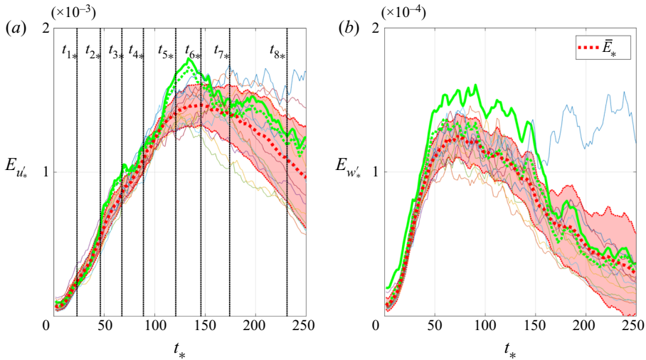
Figure 3. Energy evolution of (a) streamwise ( u'_* ) and (b) spanwise ( w'_* ) velocity fluctuations for Re = 520 and A = 60 . The red dashed curve represents the energy evolution \overline{E}_* averaged over all realizations. In (a) eight subsequent instants are marked by black vertical lines and denoted by t_{i*} , where i = 1, 2, \dots, 8 . The maximal energy gain \overline{E}_{u'_*} is reached at t_{6*} . Other instants have been selected such that \overline{E}_{u'_*}(t_{1*}) = 0.2 \max(\overline{E}_{u'_*}) , \overline{E}_{u'_*}(t_{2*}) = 0.4 \max(\overline{E}_{u'_*}) , \overline{E}_{u'_*}(t_{3*}) = 0.6 \max(\overline{E}_{u'_*}) , \overline{E}_{u'_*}(t_{4*}) = \overline{E}_{u'_*}(t_{8*}) = 0.75 \max(\overline{E}_{u'_*}) and \overline{E}_{u'_*}(t_{5*}) = \overline{E}_{u'_*}(t_{7*}) = 0.95 \max(\overline{E}_{u'_*}) . The instants t_{1*} – t_{8*} correspond to the instantaneous velocity fields presented in figure 2. The green solid curve represents the realization during which some additional small patch of turbulence that travelled from the test section was located within the area of measurements. The green dotted curve corresponds to the same realization as the solid green curve but after removing this additional patch of turbulence. The red semi-transparent area on each plot indicates the region bounded by \overline{E}_*(t_*) \pm \text{std}(E_*(t_*)) .
