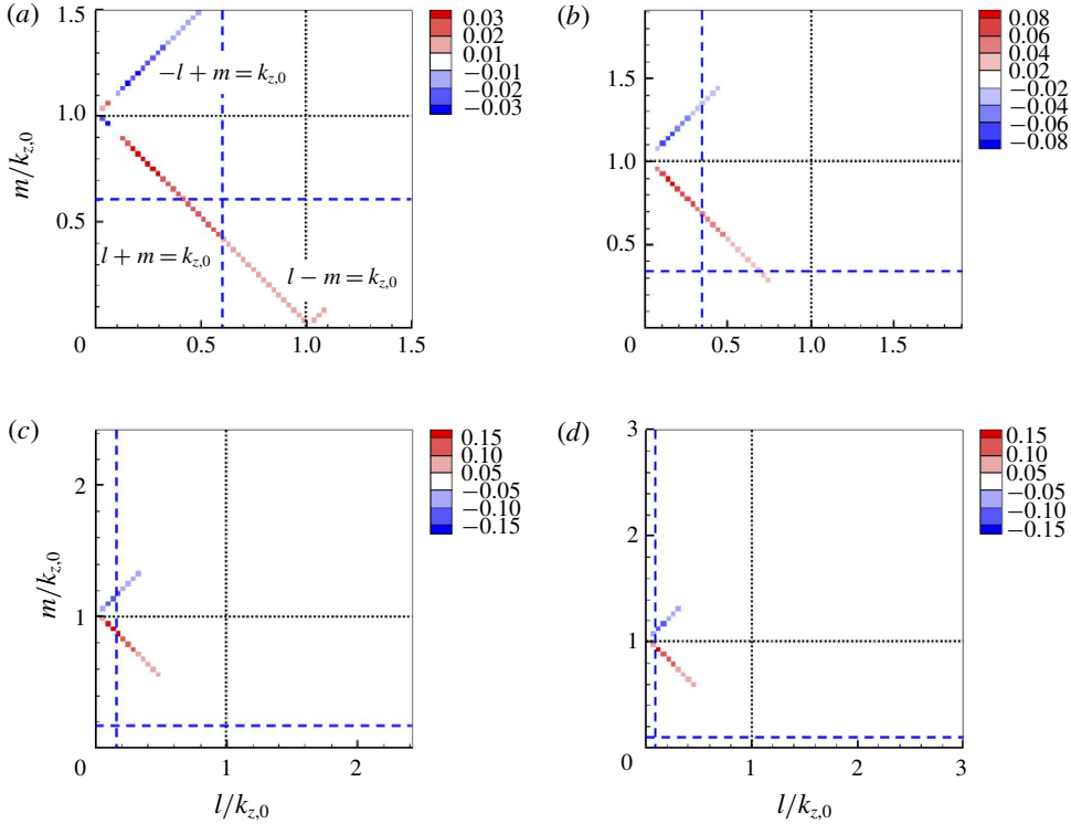
FIGURE 6. (Colour online) Triadic interactions ( \widehat{T}_{urb} ) at the locations of black dots along \lambda_z = 57\eta in figure 5(a): (a) y_0^+ = 67 ( y_0/h = 0.04 ); (b) y_0^+ = 157 ( y_0/h = 0.09 ); (c) y_0^+ = 391 ( y_0/h = 0.23 ); (d) y_0^+ = 1033 ( y_0/h = 0.62 ). Here, the black and blue dashed lines correspond to l = m = k_{z,0} and l = m = 2\pi/(3y_0) , respectively (figure 4), and the positive (red) and negative (blue) colours indicate the values of energy influx and outflux in the summation notation of (3.1), respectively.
