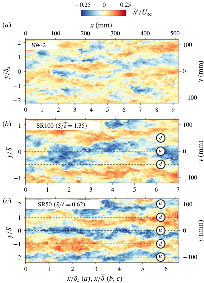
FIGURE 16. Snapshot of \tilde{u}' (turbulent fluctuations and mean spanwise variation) for (a) the reference smooth-wall case SW-2, (b) SR100 and (c) SR50, taken from WPPIV measurements. Dashed lines are the spanwise locations related to the common flow up (u) and common flow down (d) of the mean secondary flows.
