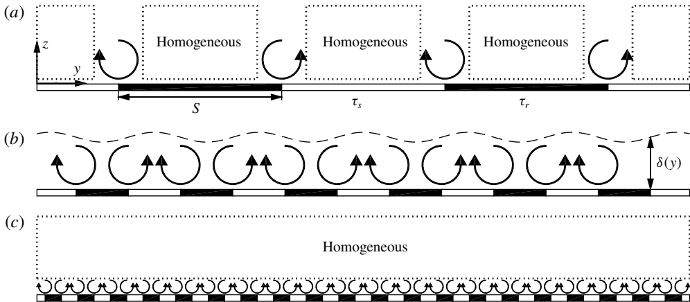
FIGURE 2. Illustration of surfaces with spanwise heterogeneous roughness, similar to that shown in Chung et al. (2018): (a) limiting case S/\delta \gg 1 , (b) intermediate case S/\delta \approx 1 and (c) limiting case S/\delta \ll 1 . The boundary-layer thickness is ---; areas bounded by ..... show regions approaching spanwise homogeneity.
