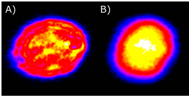
Figure 9. (A) Near-field mode of laser pulse input onto the plasma mirror. (B) Near-field mode of laser pulse after reflection from the plasma mirror. Note the smoothing of the mode performed by the plasma mirror.
