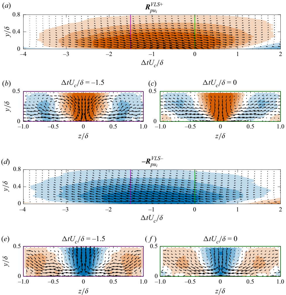
Figure 13. Visualizations of the vector fields associated with (a–c) R_{pu_i}^{VLS+} and (d–f) -R_{pu_i}^{VLS-} . The background colour represents the streamwise component of the correlations and has the same scaling as figure 12(a). The coloured lines in (a,d) show the locations of the spanwise–wall-normal planes that are plotted directly below. The vector lengths in (b,c,e,f) have been altered relative to those in (a,d) to improve the visualizations.
