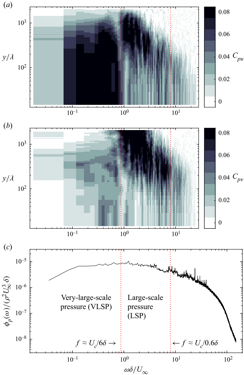
Figure 9. Estimated coherence between wall pressure and velocity fluctuation ( C_{pu_i} ) as a function of wall-normal distance as defined by (4.1) for the (a) streamwise and (b) wall-normal velocity components. Computed using the high-speed PIV measurements from FOV2. The power spectral density ( \phi_p(\omega) ) normalized by outer-layer variables is shown in (c) with the frequency axis aligned for reference.
