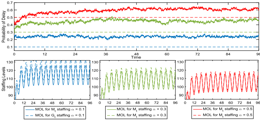
FIGURE 5. Estimated PoD for the H_2^t(1,4)/LN(1,4)/s_t model with z = 2.11 using the MOL staffing algorithm in (3.1) with z = 1 as would be done for the same model with an M_t arrival process, for targets \alpha = 0.1, 0.3, 0.5 (above) and comparison of the associated staffing levels using the MOL staffing for H_2^t(1,4) and M_t arrivals (below).
