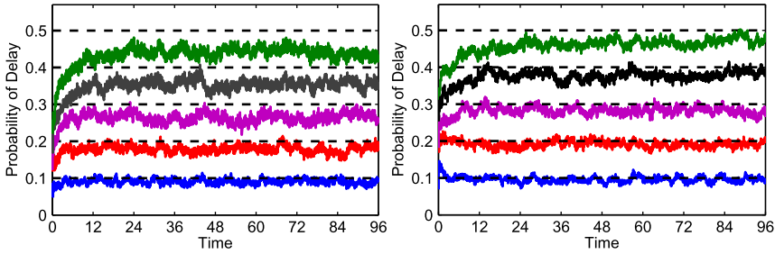
FIGURE 13. Estimated time-varying PoD for the M_t/M/s_t model ( z = 1 , left) and the H_2^t(1,4)/LN(1,4)/s_t model ( z = 2.11 , right) using the MOL SRS formula (3.1) for five delay probability targets \alpha .
