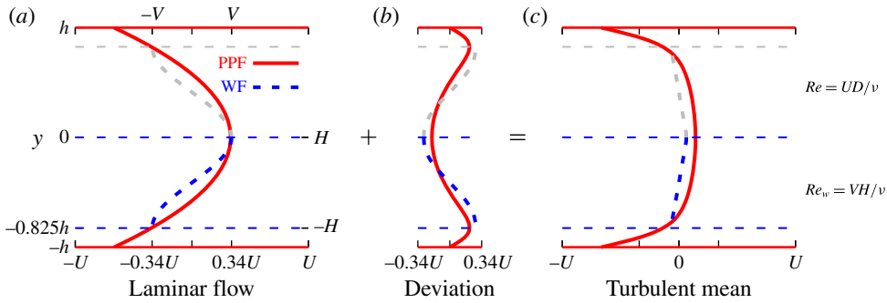
FIGURE 6. Doubled Waleffe flow seen as an approximation to the interior of plane Poiseuille flow. Shown are streamwise velocity profiles for PPF (solid/red) and WF (dashed/blue and grey) in the uniformly turbulent regime (PPF: Re = 1800 and WF: Re_w = 500 ). Plotted are (a) laminar flow and (b) deviation of mean turbulent profile from laminar flow and (c) mean turbulent profile. The y-scale of WF is non-dimensionalised using H = 2h/0.825 to align its stress-free boundaries (dashed horizontals) with extrema of the PCF deviation profile in (b). WF velocities are likewise scaled by V = 2U/0.825^2 so that both flows have same average laminar shear in (a). Data are from simulations of 2000 advective time units for [L_x, L_y, L_z] = [12, 2, 10]h .
