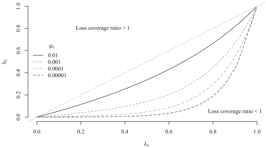
FIGURE 5: Curves demarcating the regions where LCR is greater than and less than 1 for different values of \mu_1 when \alpha_1 = 0.9 and \mu_2 = 0.04 .
