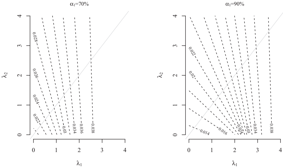
FIGURE 2: Equilibrium premium as a function of (\lambda_1, \lambda_2) for \alpha_1 = 70\% and \alpha_1 = 90\% , when (\mu_1, \mu_2) = (0.01, 0.04) .
