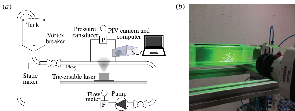
FIGURE 3. (Colour online) (a) Schematic of the flow loop. (b) Photo of the section where PIV is performed.
