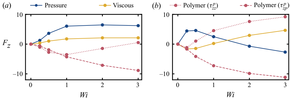
FIGURE 11. Net force contributions acting in the swimming ( z ) direction in the case of (a) \zeta = 0 and (b) \zeta = 5 when using the FENE-P constitutive equation ( L = 5, \beta = 0.5 ). The polymer stress contribution, F_z^{poly} = \int_S \tau_{zj}^p n_j dS , is broken down into portions related to normal polymeric stresses ( \tau_{zz}^p ) and shear polymeric stresses ( \tau_{z\rho}^p ).
