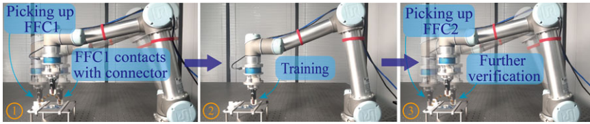
Figure 8. The procedure of the FFC assembly experiment.
