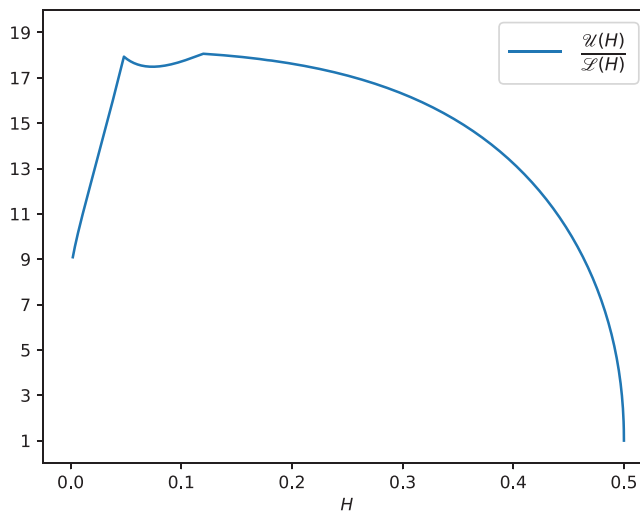
FIGURE 3: The ratio between the upper and lower bounds for \mathcal{M}(H) for H \in [0, \frac{1}{2}] .
