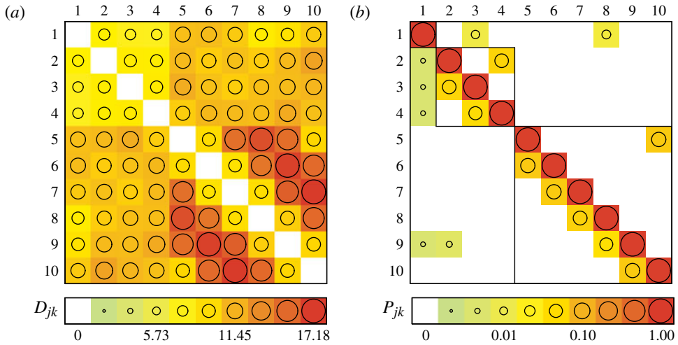
FIGURE 15. (Colour online) Kinematics and dynamics: (a) distance matrix \mathbf{D} and (b) transition matrix \mathbf{P} of the clustered mixing layer data (see figure 13). Values are displayed as in figure 4.
