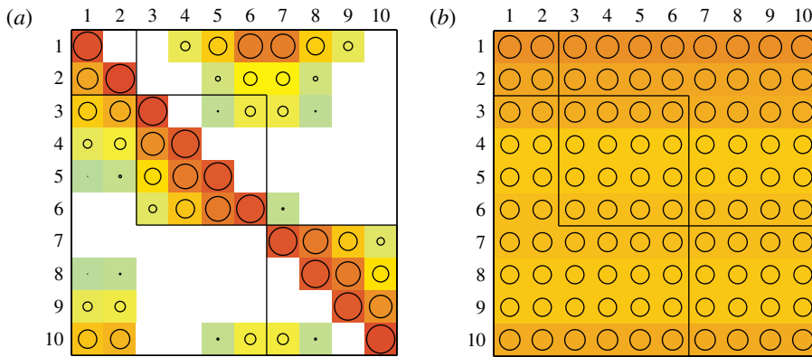
FIGURE 6. (Colour online) Dynamics of the clustered Lorenz attractor illustrating (a) l = 10 and (b) l = 1000 iterations of the transition matrix \mathbf{P} . The matrices are visualised like in figure 4(b). Note that the increasing iterations make the matrices \mathbf{P}^l more uniform.
