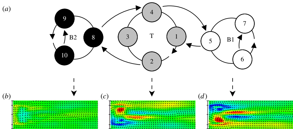
FIGURE 28. (Colour online) Simplified cluster transitions (analogous to figure 16). The arrows indicate possible transitions above a certain threshold. This threshold is chosen small enough to guarantee full connectivity. The graph highlights three cyclic groups associated with the two asymmetric bimodal states and a transition region between them. Two branching clusters, k=5 and k=8 , connect these groups. Mean velocity fields of the three cluster groups of Ahmed body are shown below: (b) bimodal group ‘B2’ of clusters k=8, 9, 10 , (c) symmetric group ‘T’ of clusters k=1, 2, 3, 4 , (d) bimodal group ‘B1’ of clusters k=5, 6, 7 . The visualisation of the mean flows corresponds to those in figure 27.
