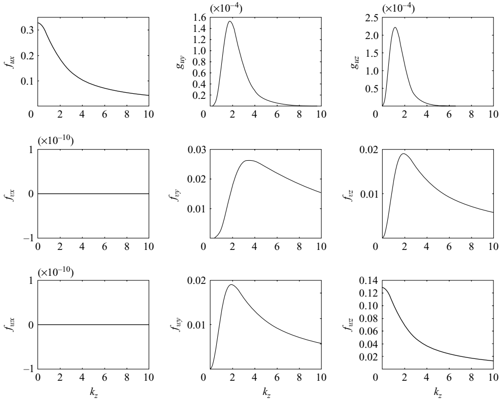
FIGURE 7. Plots of f_{rs}(k_z) , \{r = u, v, w; s = x, y, z\} , g_{uv}(k_z) and g_{uz}(k_z) . Functions g_{uv}(k_z) and g_{uz}(k_z) are determined for Couette flow.
