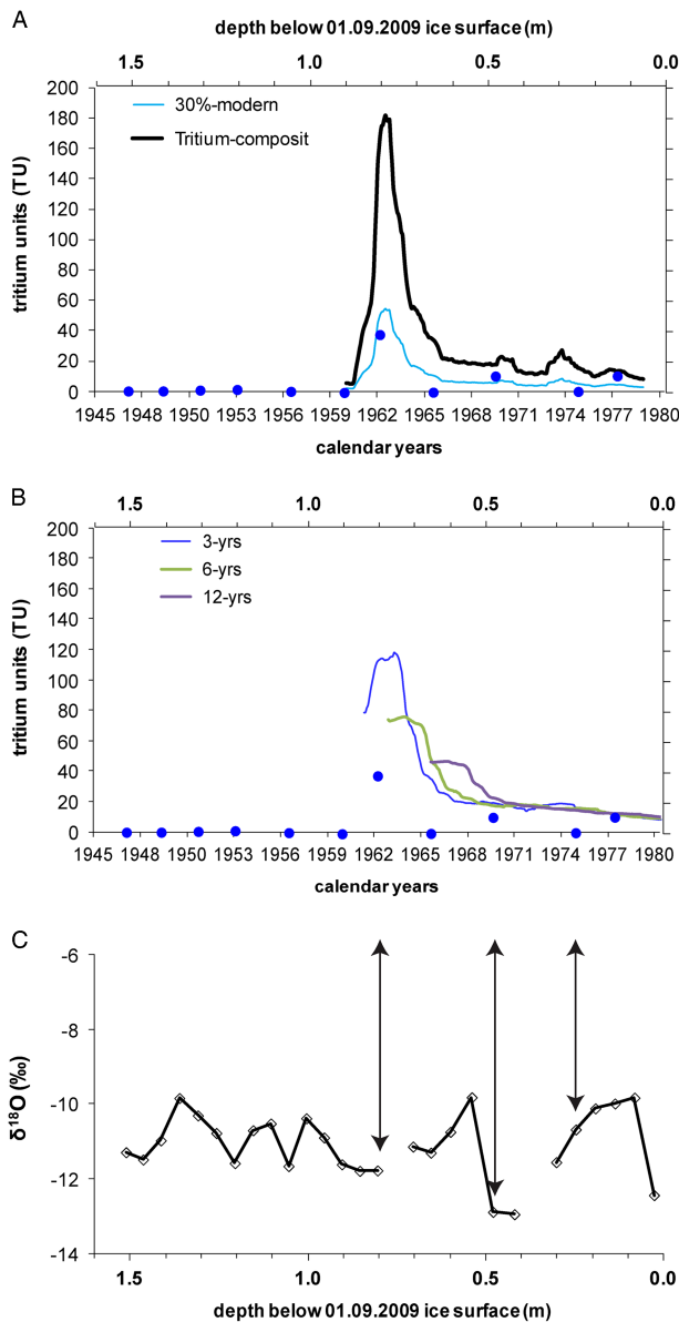
Figure 2 ^3\text{H} activity in regional precipitation (composite of monthly data from Feuerkogel and Vienna and decay corrected to 01.09.2009) and Saarhalle ice core obtained using the ^3\text{He} -ingrowth method (blue dots). A: decay corrected annual mean ^3\text{H} activities of precipitation (black) and the dampened signal assuming constant mixing of 30% modern precipitation and 70% tritium-free old water. B: decay corrected monthly ^3\text{H} activities of precipitation smoothed with 3-yr (blue), 6-yr (green), and 12-yr (purple) moving averages simulating multiannual mixing in the karstic reservoir during the infiltration process. C: stable oxygen isotope composition of the cave ice samples in the upper 1.5 m section of the Saarhalle ice core (Kern et al. 2011). (See online version for colors.)
