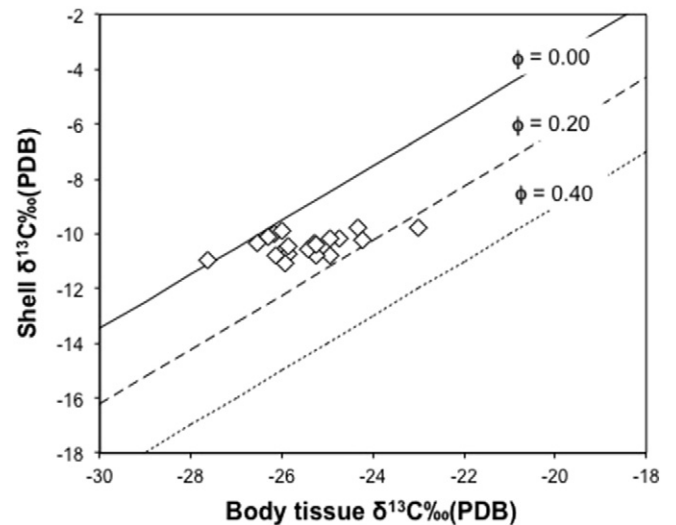
Figure 5. Calculated curves of land snail shell \delta^{13}\text{C} values as a function of body \delta^{13}\text{C} values, which depict snail's diet, based on the steady-state flux balance model by Balakrishnan and Yapp (2004). Calculations were made assuming that calcification occurred at average air temperatures of 13^\circ\text{C} .
