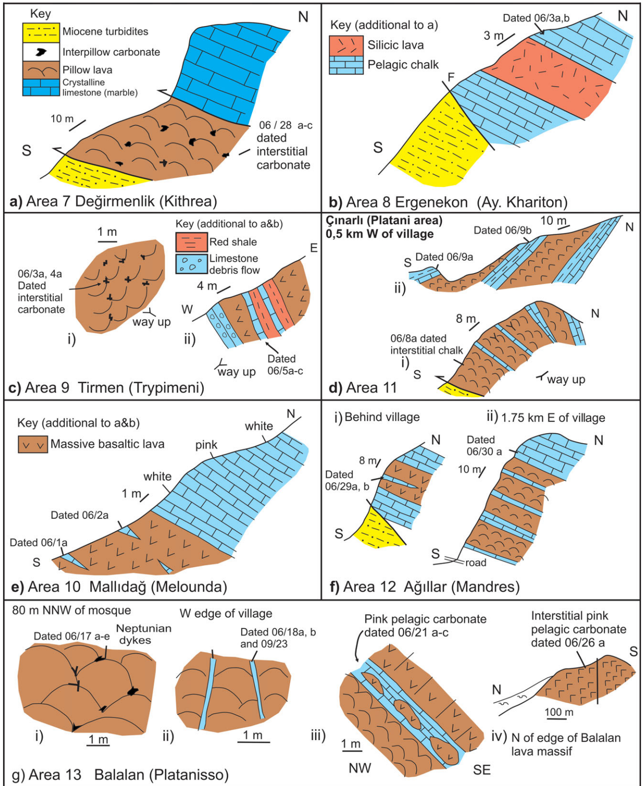
Figure 11. (Colour online) Field relations of dated chinks associated with basaltic lavas in the central and eastern Kyrenia Range, areas 7–13. See text for an explanation of each area. The locations of samples are listed in Tables A1 and A2.
