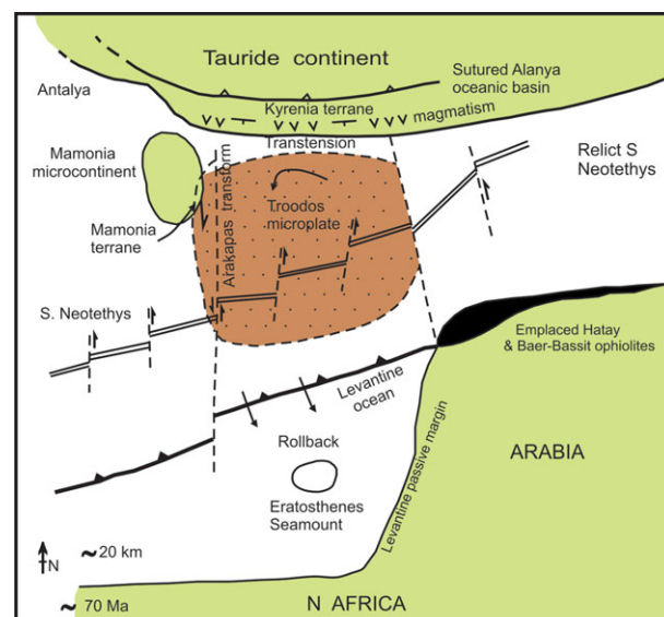
Figure 15. (Colour online) Plate tectonic interpretation showing the possible relation of the Kyrenia Range (Kyrenia terrane) to the anticlockwise rotation of the Troodos microplate during Late Cretaceous–Palaeogene time. Based on Robertson (1990) and Inwood et al. (2009). In an alternative tectonic model some oceanic crust still remained between the microplate and the Kyrenia margin; see text for explanation.
