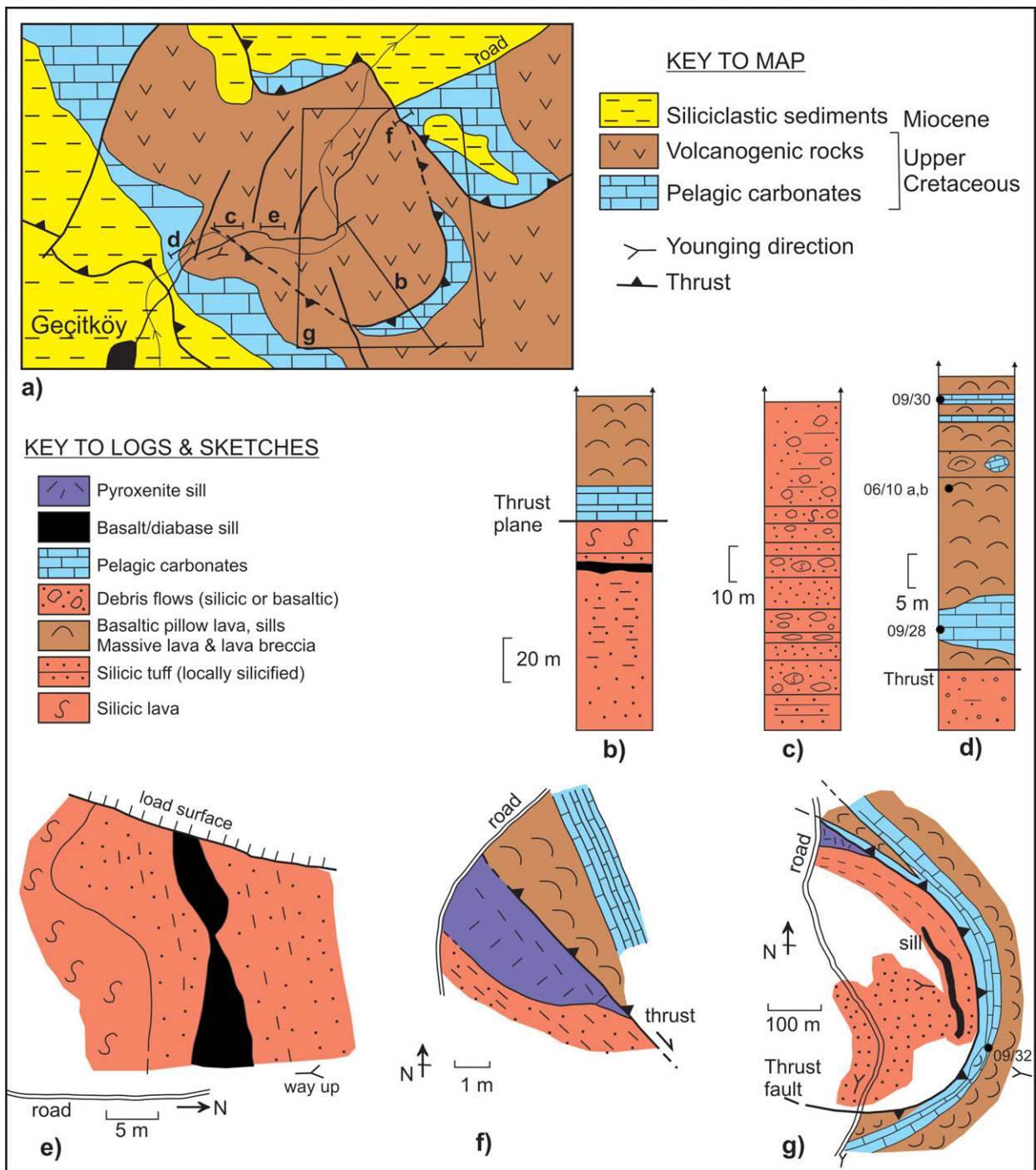
Figure 8. (Colour online) Field relations of Upper Cretaceous volcanic and sedimentary rocks exposed near Geçiköy (Panagra) in the western Kyrenia Range (Area 2 in Fig. 1). (a) Outline geological map based on Baroz (1979), Moore (1960) and this work. The area is dominated by a recumbent SE-verging anticline of inferred Late Miocene–earliest Pliocene age. (b) Measured log of the section marked b on the map in (a). The lower part comprises well-bedded tuff with coarser and finer interbeds (< 0.5 m thick) and rare tuffaceous debris flows (clasts < 2 cm in size). The thrust plane is characterized by small duplexes of basalt entrained along the contact. (c) Local log of part of the silicic volcanogenic sequence exposed along the main road. This begins with a volcanic conglomerate with mainly sub-rounded to sub-angular boulders of hard flinty rhyolite in a pale, chaotic debris-flow unit. The sequence grades upwards into relatively massive white tuff with scattered small lava clasts. Overlying thick debris flows include angular clasts of grey flinty rhyolite clasts (up to 2.5 m in size). Interbedded fine-grained tuff contains scattered rhyolite blocks (up to 0.8 m in size). (d) Local log of basalt and pelagic chalk sequence exposed in the road section, structurally above the silicic volcanogenic sequence (see (c)). The chalk is interbedded with pillow basalt, lava breccia and hyaloclastite mixed with chalk. Chalk interbeds are dated as Late Campanian–Maastrichtian (sample 09/28) and as Late Maastrichtian (sample 06/10a, b), while pelagic limestone interbedded with pillow basalt along the road section to the south is dated as Middle Eocene (sample 09/30). (e) Part of the sequence along the north side of the main road exposes weakly bedded silicic tuff, locally overlain by a vitreous rhyolite flow. A small irregular body interpreted as a high-level basaltic intrusion cuts the tuff. (f) Pyroxenite sill intruding tuffaceous sediments. The intrusion is truncated by a thrust, above which comes a contrasting succession of Upper Cretaceous pelagic chalk and basalt. (g) The lower silicic lava/tuff sequence and the overlying Upper Cretaceous pelagic chalk/basalt sequence are separated by a thrust. Both sequences are folded into a SE-facing anticline of Late Miocene–earliest Pliocene age.
