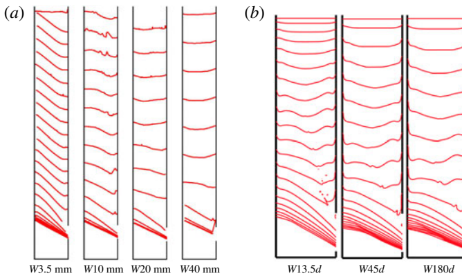
FIGURE 11. (Colour online) Profiles of the top surface of granular materials for various W at constant time steps: (a) experiments with D = 25 mm, d = 190 \mu m, time interval \Delta t_e = 0.5 s, (b) continuum simulation with D = 56.25d and time interval \Delta t_s/\sqrt{d/g} = 9.5 .
