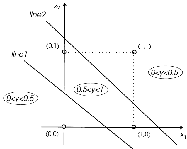
Figure 1 (Damper). Possible separating "hyperplanes" for the 2-input parity problem, corresponding to the decision boundaries formed by the two hidden units. In this simple case, the hyperplanes are lines.
