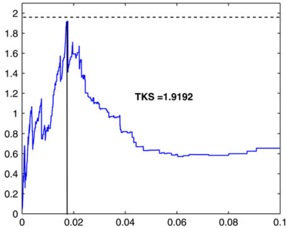
FIGURE 1. Plot of \{\hat{\sigma}\sqrt{0.99}\}^{-1}|\widehat{\mathcal{W}}_n(y)| against y for squared log returns of Intel stocks. The horizontal dashed line corresponds to the 10% level critical value of the TKS test. The observed test statistic \text{TKS} = 1.9192 is the supremum of the curve.
