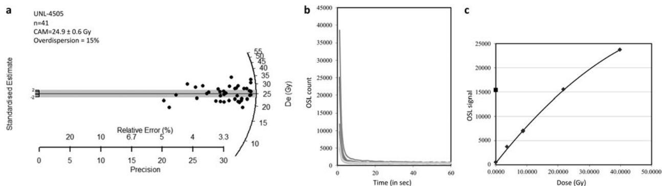
Figure 5. Diagrams showing optically stimulated luminescence (OSL) data for sample UNL-4505 from Munn 4: (a) radial plot of equivalent dose (D e ) values; (b) OSL shinedown curve; (c) SAR dose response curve.
