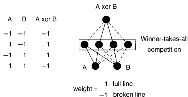
Figure 10. A network that performs the XOR mapping.
