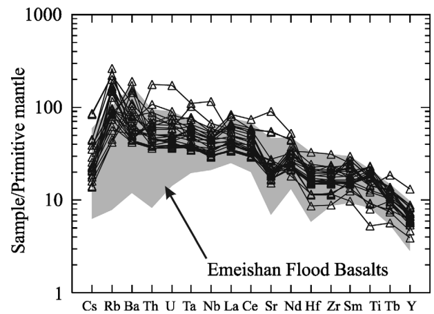
Figure 7. Primitive-mantle-normalized trace element data patterns plots of the mafic dykes and Emeishan flood basalts normalized to values of Sun & McDonough (1989). Flood basalt data from Song et al. (2001, 2004) and Xu et al. (2001).
