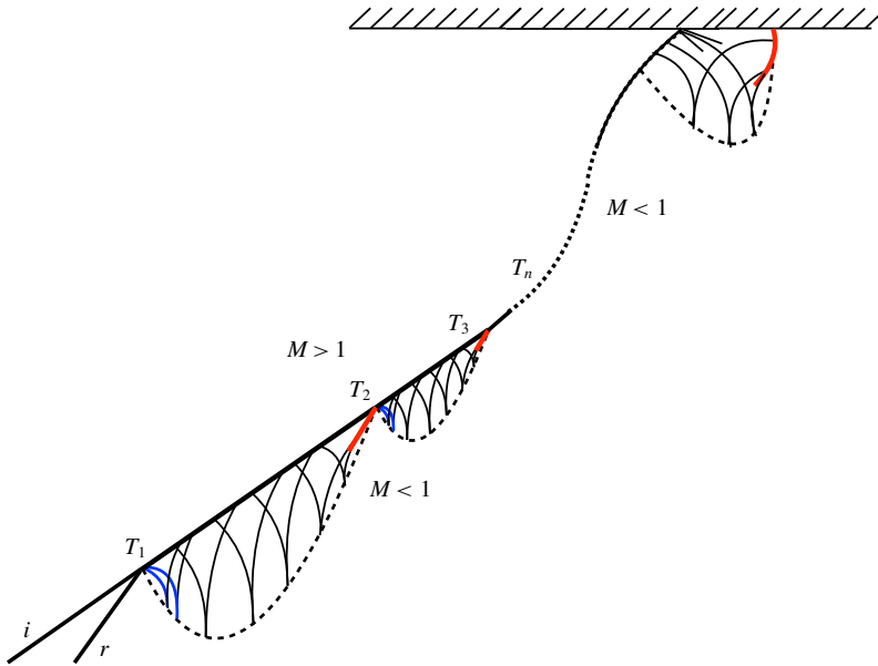
FIGURE 19. (Colour online) Sketch of flow scenario associated with a sonic Mach stem generating a supersonic pocket attached to the reflecting channel wall and terminating in an upstream shock.
