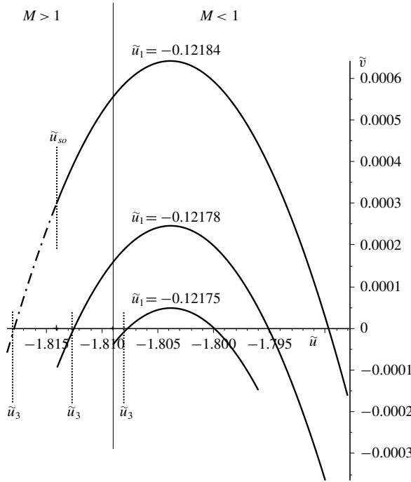
FIGURE 11. Section of reflection polar K_1 > 0 , -1/K_1 < K_2 < -3/4K_1 . Results are for K_1 = 1, K_2 = -0.8 . The transition is shown to a compound shock/fan structure as the wedge angle increases (or \tilde{u}_1 decreases) leading to the downstream state \tilde{u}_3 .
