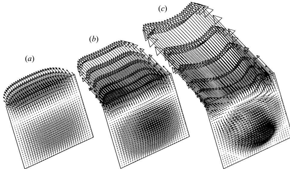
FIGURE 15. Thermocapillary steady flow solutions without a magnetic field ( Ha = 0 ). The velocity vectors are plotted in the (Tv)-plane for three Reynolds numbers: (a) Re = 5 \times 10^2 ; (b) Re = 2 \times 10^3 and (c) Re = 5 \times 10^3 .
