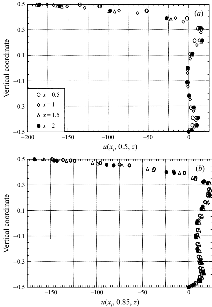
FIGURE 19. Thermocapillary steady flow solution for the B_x case at Re = 2 \times 10^3 and Ha = 200 . The horizontal velocity profiles along z are given at various longitudinal locations ( x = 0.5, 1, 1.5 and 2 ) and for two transversal locations: (a) y = 0.5 and (b) y = 0.85 .
