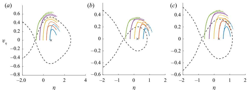
FIGURE 20. Trajectories near the leading edge for: (a) Mach 10, 10° ramp and initial sphere locations of x_0/r = 5, 9, 13, 17 and 21; (b) Mach 6, 10° ramp and initial sphere locations of x_0/r = 3, 5, 7, 9 and 11; (c) Mach 6, 15° ramp and initial sphere locations of x_0/r = 3, 5, 7, 9 and 11. In each case, the solid lines show the results of free-flight simulations and the dot-dashed lines indicate the predicted trajectory from the decoupled force model.
