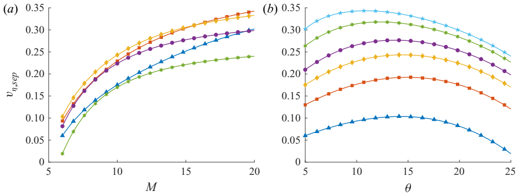
FIGURE 12. Normalized shock relative velocity when the sphere is free of the wall influence: (a) versus Mach number for ramp angles of ( \text{---}\blacktriangle\text{---} ) 5^\circ , ( \text{---}\blacksquare\text{---} ) 10^\circ , ( \text{---}\blacklozenge\text{---} ) 15^\circ , ( \text{---}\bullet\text{---} ) 20^\circ and ( \text{---}\blacktriangledown\text{---} ) 25^\circ ; and (b) versus ramp angle for Mach numbers of ( \text{---}\blacktriangle\text{---} ) 6, ( \text{---}\blacksquare\text{---} ) 8, ( \text{---}\blacklozenge\text{---} ) 10, ( \text{---}\bullet\text{---} ) 12, ( \text{---}\blacktriangleleft\text{---} ) 16 and ( \text{---}\blacktriangleright\text{---} ) 20.
