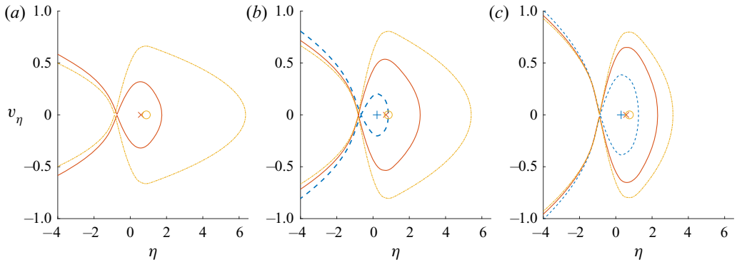
FIGURE 5. Separatrices of the phase diagrams for a sphere interacting with a ramp-generated oblique shock for ramp angles of (a) 5°, (b) 10° and (c) 20°, in each case for free-stream Mach numbers of (---) 6, (—) 10 and (- · - · -) 20. The symbols indicate the centre locations for (+) Mach 6, (x) Mach 10 and (o) Mach 20.
