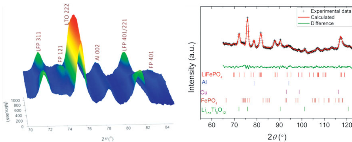
Figure 3. (Color online) Waterfall plot (left) of a collection of NPD patterns shown for a restricted 2\theta range taken during battery charge and discharge. Labels are phase reflections for \text{LiFePO}_4 (LFP), \text{FePO}_4 (FP), \text{Li}_{4+2}\text{Ti}_5\text{O}_{12} (LTO), and Al. A typical Rietveld-refinement profile before cycling (right) is also shown. The figures-of-merit for the refinements were in the range \chi^2 = 3.9\text{--}8.95 , R_{\text{wp}} = 14.3\text{--}17.1 , and R_{\text{B}} = 1.0\text{--}3.9\% .
