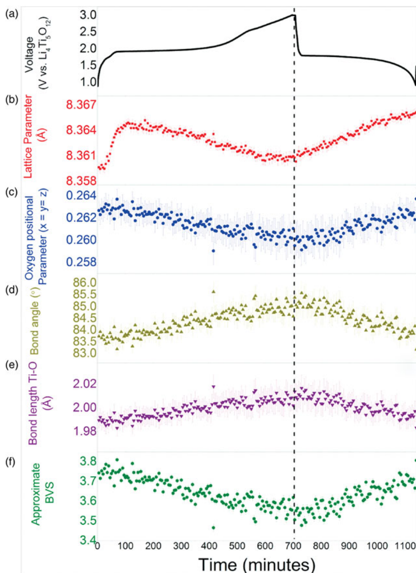
Figure 4. (Color online) (a) Charge–discharge profile, (b) refined anode lattice-parameter, (c) refined oxygen positional-parameter, (d) \alpha bond-angle, and (e) Ti–O bond length, during battery charge and discharge. The titanium oxidation-state in (f) is estimated using the approximate BVS method.
