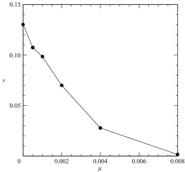
FIGURE 4. The decay of the inverse cascade strength r for the dissipation term -6 \times 10^{-6} \Delta^2 \psi + \mu \Delta \psi as \mu is increased.
