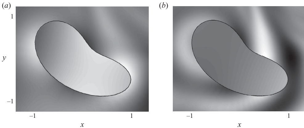
FIGURE 3. The displacement of crooked egg-shaped floes and the surrounding diffracted wave fields. The incident wave propagates along the x -axis from x \rightarrow -\infty and the (non-dimensional) free-surface wavelength \lambda = 2\pi/k_0 is 2 in (a) and 1 in (b).
