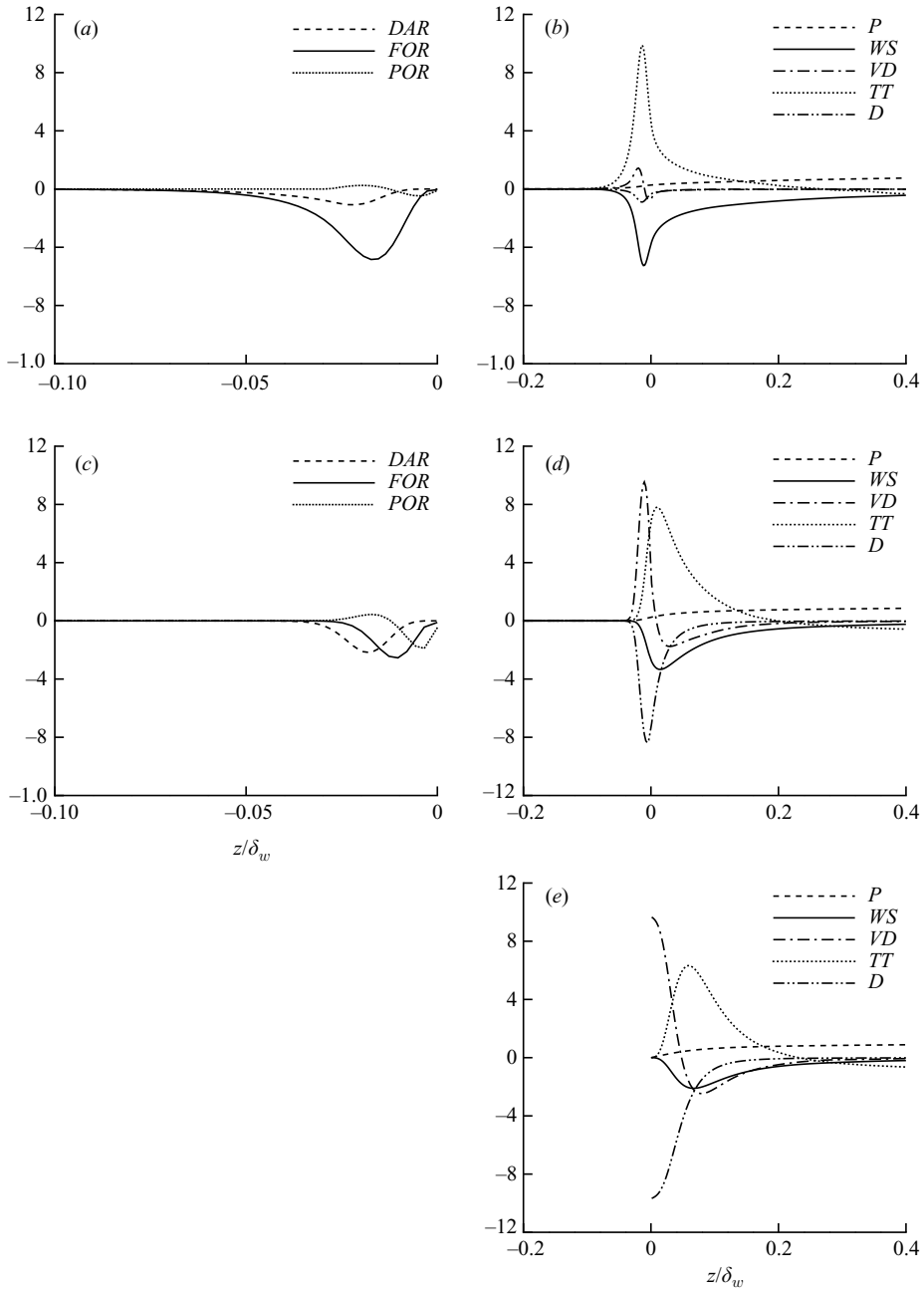
FIGURE 10. Terms in the transport equation for the mean kinetic energy \bar{u}^2/2 for different wall porosities, normalized by U_m [(u'_t)^2 + (u'_l)^2]/H and shown as function of z/\delta_w . (a, b) case E95; (c, d) case E80; (e) case E0.
