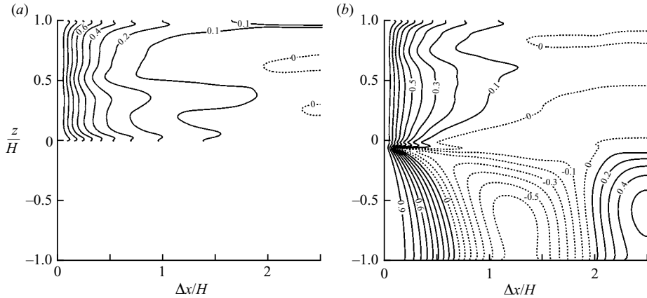
FIGURE 23. Isocontours of the autocorrelation \rho_{u'u'} as a function of the streamwise spacing \Delta x/H , and shown across the permeable wall and the channel. The solid and dashed lines correspond to, respectively, positive and negative values of \rho_{u'u'} , with a step of 0.1 between two neighbouring lines. (a) Case E0; (b) Case E95.
