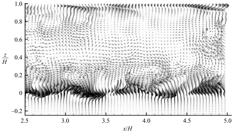
FIGURE 4. Two-dimensional snapshot of an instantaneous flow field ( u', w' ) in case E95. Note that the lower part of the permeable wall is not shown, because velocities in this region are much smaller than in the channel region.
