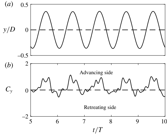
FIGURE 20. Time trace of the total lift coefficient, C_y (b), correlated with the displacement signal (a) for \alpha = 0.7 at U^* = 6 . Asymmetry in the force signal as the sphere traverses from the advancing to the retreating side is evident in the time trace.
