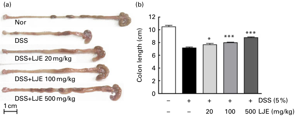
Fig. 3. Effects of the water extract of Lonicera japonica (LJE) on colon length in dextran sulphate sodium (DSS)-induced colitis. (a) Representative images of a typical colon morphology and the length of each group. (b) A graph showing the data of colon length. Values are means ( n = 8 for each group), with their standard errors represented by vertical bars. Mean values were significantly different compared with the DSS group: * P < 0.05 , *** P < 0.001 . Nor, normal group; DSS, a group treated with DSS; DSS + LJE, DSS group treated with each dosage of the water extract of Lonicera japonica (a colour version of this figure can be found online at www.journals.cambridge.org/bjn ).
