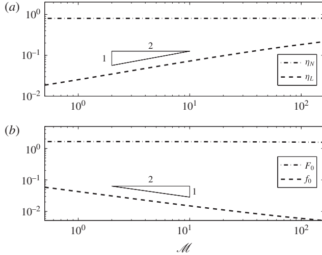
FIGURE 15. (a) Front positions and (b) source thicknesses of two dimensional currents on log–log axes versus viscosity ratio, for \mathcal{D}=0.001 and \mathcal{D}=1 , corresponding to regime (I). The power laws (5.1a–d) for \eta_L and f_0 with respect to \mathcal{M} are shown as triangles.
