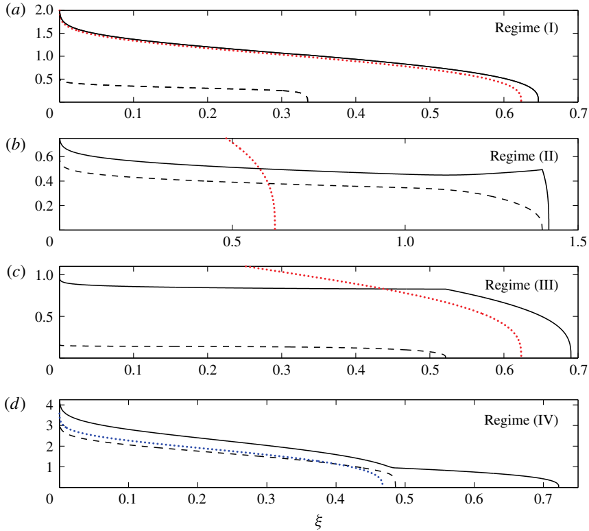
FIGURE 13. (Colour online) Profile thicknesses of axisymmetric two-layer gravity currents in similarity coordinates for a range of different parameters with \mathcal{D} = 1 fixed. Upper surface heights are solid and interfacial heights are dashed. The dotted (red online) curves in (a–c) are the surface heights that the upper fluid would have if the lower fluid were not present. The dotted (blue online) curve in (d) is the surface height that the lower fluid would have if the upper fluid were not present. The parameter values used are \mathcal{M} = 1 , \mathcal{Q} = 0.1 in (a), \mathcal{M} = 100 , \mathcal{Q} = 2 in (b), \mathcal{M} = 100 , \mathcal{Q} = 0.1 in (c), and \mathcal{M} = 0.05 and \mathcal{Q} = 1 in (d). (a–d) correspond to regimes (I)–(IV), respectively.
