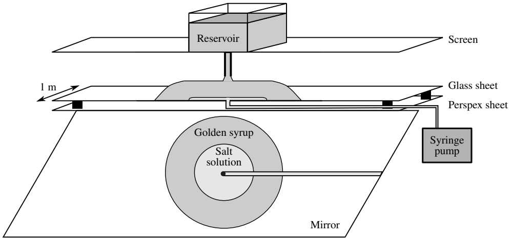
FIGURE 6. Schematic of our experimental set-up.
