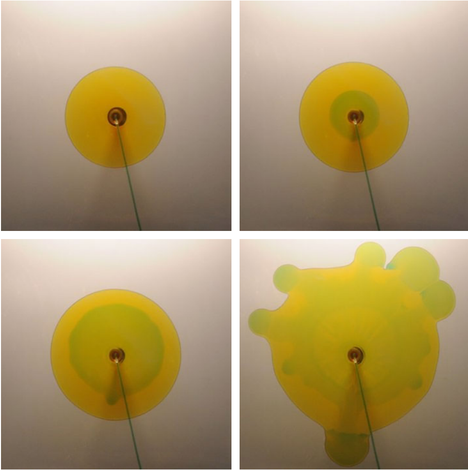
FIGURE 7. Bottom view of experiment D at t = 0, 60, 180, 420 s after injection of salt solution. The full experiment is shown in supplementary movie 1 ( http://dx.doi.org/10.1017/jfm.2015.30 ).
