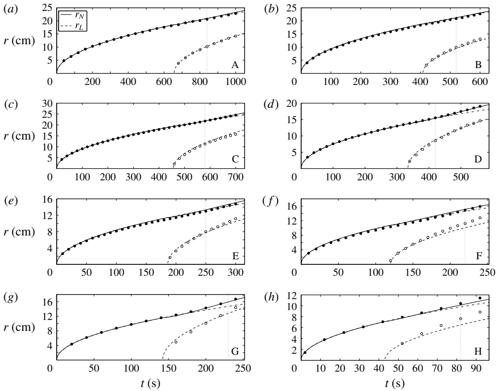
FIGURE 9. Comparison of our experimental data for experiments A–H for r_N (filled symbols) and r_L (open symbols) to solutions for r_N (solid) and r_L (dashed) of the full system of PDEs (3.8)–(3.16) for axisymmetric spreading. The dash-dot curves show r_N as a function of t in the unlubricated case. The vertical dotted lines indicate the time at which there is a first sign of a fingering instability in the experiments.
