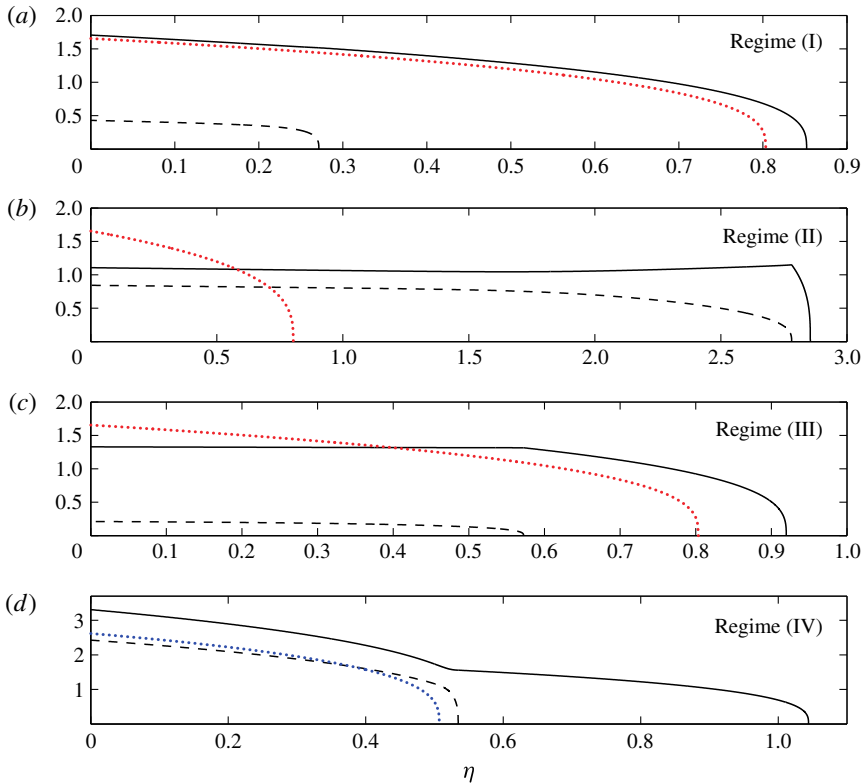
FIGURE 12. (Colour online) Profile thicknesses of two-dimensional two-layer gravity currents in similarity coordinates for a range of different parameters with \mathcal{Q} = 1 fixed. Upper surface heights are solid and interfacial heights are dashed. The dotted (red online) curves in (a–c) are the surface heights that the upper fluid would have if the lower fluid were not present. The dotted (blue online) curve in (d) is the surface height that the lower fluid would have if the upper fluid were not present. The parameter values used are \mathcal{M} = 1 , \mathcal{Q} = 0.1 in (a), \mathcal{M} = 100 , \mathcal{Q} = 2 in (b), \mathcal{M} = 100 , \mathcal{Q} = 0.1 in (c) and \mathcal{M} = 0.05 and \mathcal{Q} = 1 in (d). (a–d) correspond to regimes (I)–(IV), respectively.
