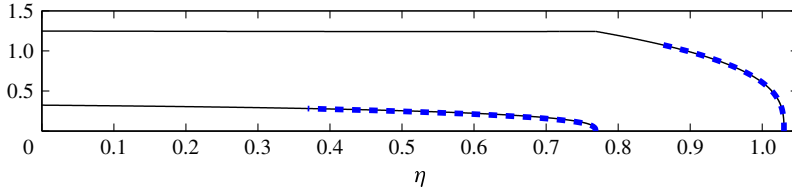
FIGURE 3. (Colour online) Similarity solutions and asymptotic results in two dimensions. Solutions of (2.38)–(2.47) for the thicknesses of both currents are presented as solid curves. Asymptotic solutions (2.48) and (2.49) near the two fronts are presented as dashed bold curves. Parameter values used are \mathcal{M} = 100 , \mathcal{D} = 1 and \mathcal{Q} = 0.2 .
