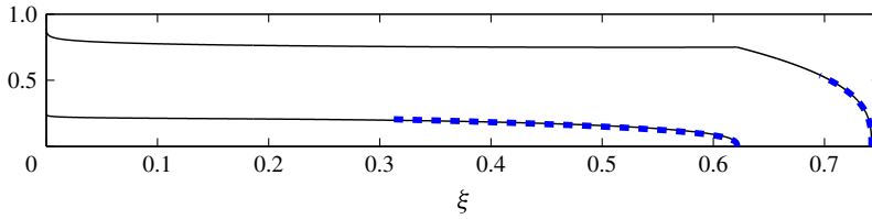
FIGURE 5. (Colour online) Similarity solutions and asymptotic results in axisymmetry. Solutions of (3.19)–(3.28) for the thicknesses of both currents are presented as solid curves. Asymptotic solutions (3.29) and (3.30) near the two fronts are presented as dashed bold curves. Parameter values used are \mathcal{M} = 100 , \mathcal{D} = 1 and \mathcal{Q} = 0.2 .
