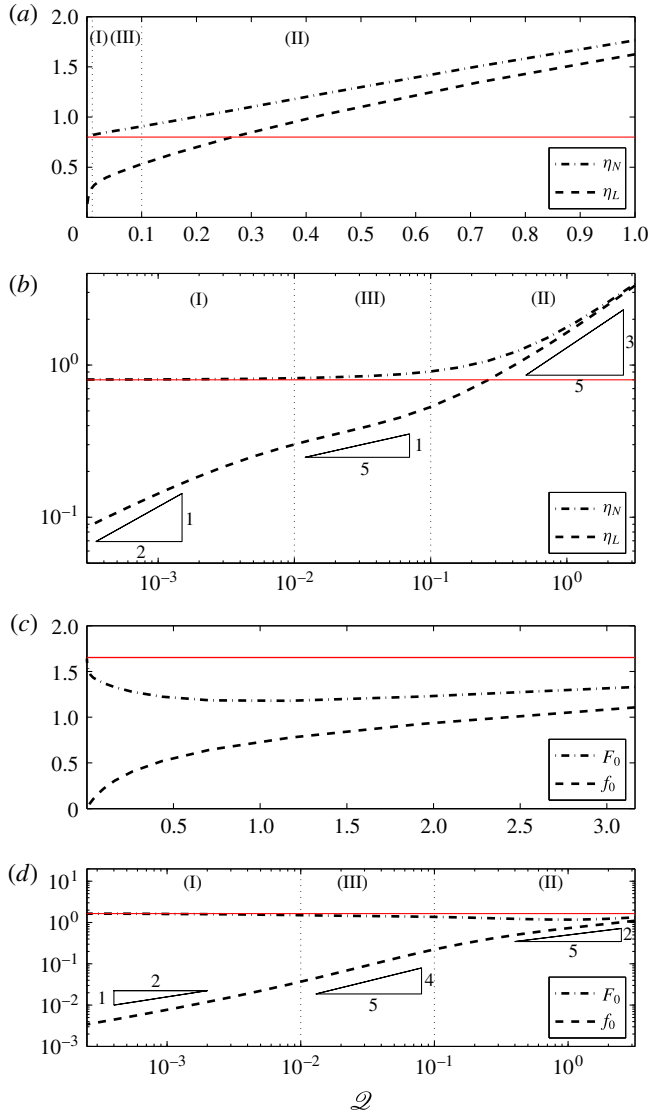
FIGURE 14. (Colour online) (a,b) Front positions and (c,d) source thicknesses of two dimensional currents on regular and log–log axes, all versus flux ratio. Parameter values used are \mathcal{M} = 50 and \mathcal{D} = 1 , corresponding to regimes (I)–(III). The solid (red online) line in (a,b) corresponds to the extent of the upper more viscous current, if the lower less viscous layer were not present. The solid (red online) line in (c) corresponds to the thickness of the upper more viscous current if the lower less viscous layer were not present. The power laws (5.1), (5.5), and (5.8) for \eta_L and f_0 with respect to \mathcal{Q} are shown as triangles.
