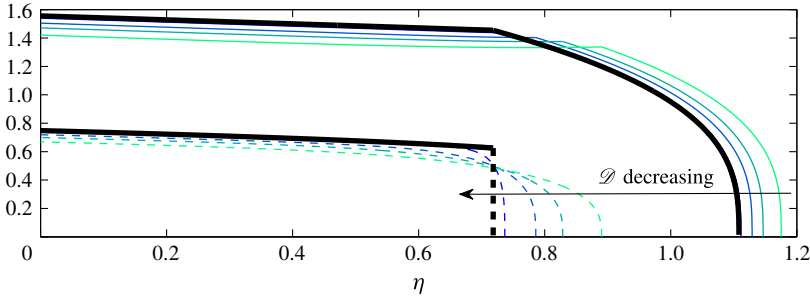
FIGURE 16. (Colour online) Two-dimensional thickness profiles in similarity coordinates for varying \mathcal{D} \in \{0.05, 0.25, 0.5, 1\} with \mathcal{M} = 10 , \mathcal{Q} = 0.5 . Surface heights are solid curves and interfacial heights between the two fluids are dashed. The \mathcal{D} = 0 singular limiting solution is shown as bold curves for the two layers.
