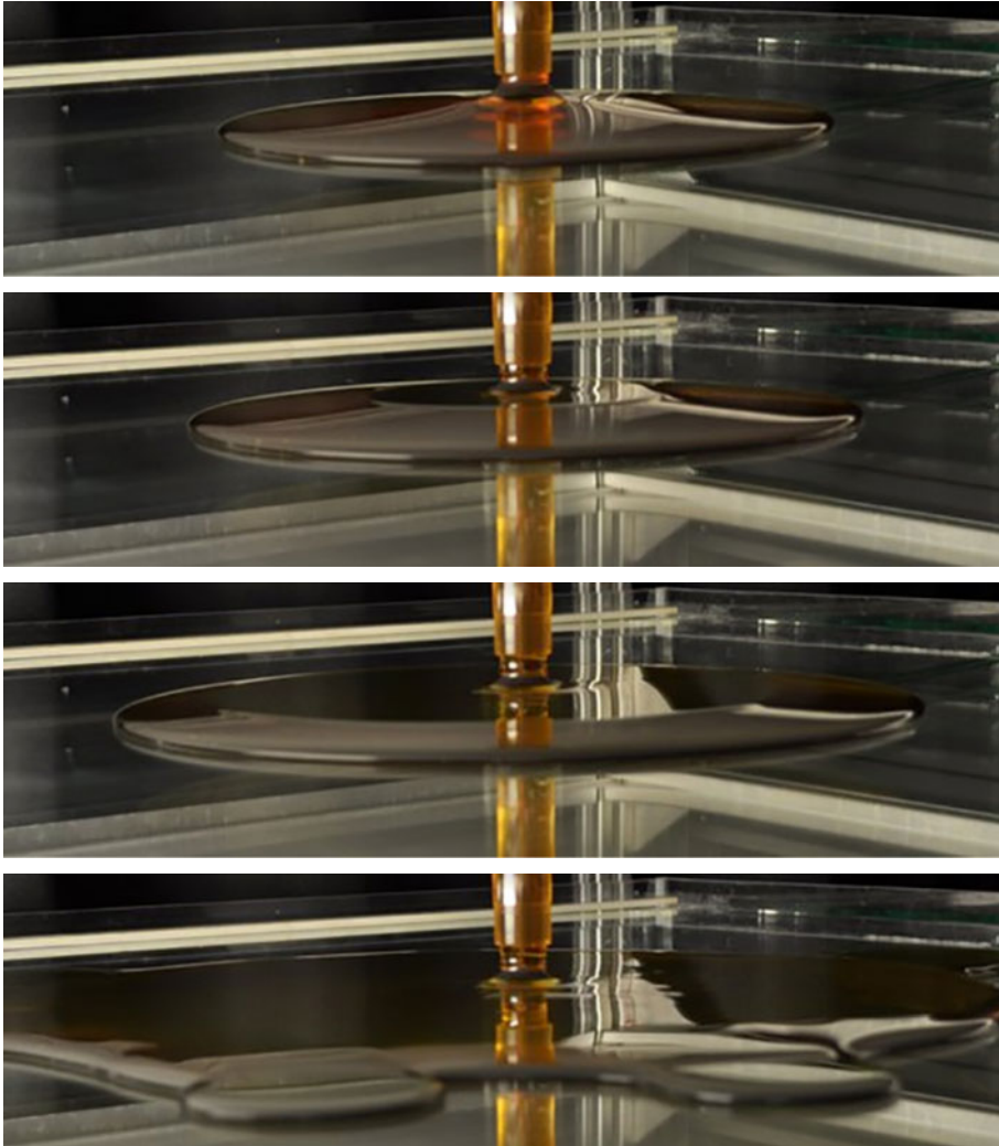
FIGURE 8. Side view of experiment D at t = 0, 60, 180, 420 s after injection of salt solution. The full experiment is shown in supplementary movie 2.
