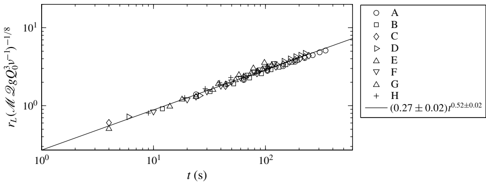
FIGURE 10. Experimental values for r_L (\mathcal{M} \mathcal{D} g Q_0^3 v^{-1})^{-1/8} versus time. The solid line is a least-squares power-law fit.
