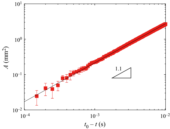
Figure 17. Time evolution of the hole area A in wetting mode II. Here, t is the time and t_0 is defined as the moment when the hole is completely closed. The red squares are experimental data with error bars, and the black solid line is the best fit to the experimental data based on the scaling law of A \sim (t_0 - t)^{1.1} .
