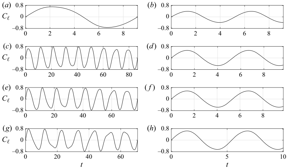
Figure 14. Time history of the lift coefficients for 4.85 \leq \mathcal{AR} \leq 5.25 in the different states. Aspect ratio \mathcal{AR} = (a,b) 4.85, (c,d) 5.0625, (e,f) 5.125 and (g,h) 5.25. (a,c,e,g) The n = 1 (bifurcated) state and (b,d,f,h) the n = 2 state. The time history of C_l is plotted over one T_{lp} period for the n = 1 bifurcated state and over one T_{TE} period for the other cases.
