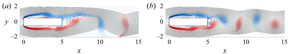
Figure 15. Snapshots of the flow around the rectangular cylinder with \mathcal{AR} = 5 , with the streamlines and vorticity colour maps, for (a) n = 1 and (b) n = 2 .
