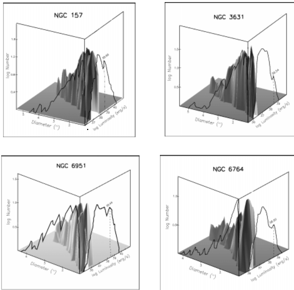
Figure 1 — H\alpha luminosity of the HII regions in four late-type spiral galaxies. The sample is complete to well below 10^{38} \text{erg s}^{-1} . The LF is obtained by projecting the number–diameter–luminosity surface into the \log N - \log L plane. Note the ‘glitch’ (change in gradient accompanied by peaks) in the LF near L = 10^{38.6} \text{erg s}^{-1} (see text for details).
