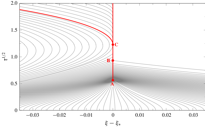
FIGURE 5. (Colour online) The characteristics corresponding to the solution shapes in figure 4, focusing on the region near the shock by using coordinates (\xi - \xi_*, \tau^{1/2}) , where \xi_*(\tau) is the shock position once it has formed and before that the radial position of the characteristic leading up to the shock. The same points of interest A to C are marked (see text).
