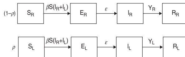
Fig. 1. Model schematic. S, Susceptible; E, exposed; I, infected; R, recovered; subscript (R), regular shedding; subscript (L), long shedding. Parameters: \beta , transmission probability; \epsilon , 1/incubation period; \gamma_R , 1/regular-shedder infectious period; \gamma_L , 1/long-shedder infectious period; \rho , fraction that is long-shedding.
