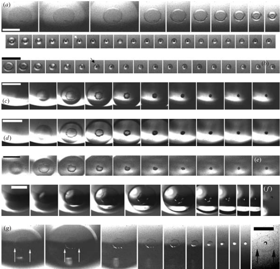
FIGURE 3. Contraction of the air disk, for various impact conditions. (a–e) Water drops D = 4.0 mm. (a) H = 9.7 cm, We = 102 , Re = 6740 , dt = 10 \mu\text{s} . (b) Images from another clip under the same conditions. The arrows point to a trumpet-shaped neck which subsequently pinches off to form a microdrop at the centre, as sketched in figure 8. (c, d) Two realizations for H = 4.4 cm, We = 44 , Re = 4420 , dt = 10 \mu\text{s} . (e) H = 8.2 cm, We = 86 , Re = 6170 , dt = 10 \mu\text{s} . (f) Drop of alcohol, H = 2.5 cm, D = 3.1 mm, We = 50 , Re = 1325 , with dt = 20 \mu\text{s} . (g) More viscous drop, 80% glycerin/water mixture, H = 11.2 cm. We \simeq 160 , Re \simeq 100 . Times shown are 0, 20, 40, 60, 80, 120, 160, 220, 320, 720, 2000 \mu\text{s} . The white arrows point out the location of the edge and the dark arrows point at a faint outer ring of micro-bubbles left behind. The scale bars are 500 \mu\text{m} long.
