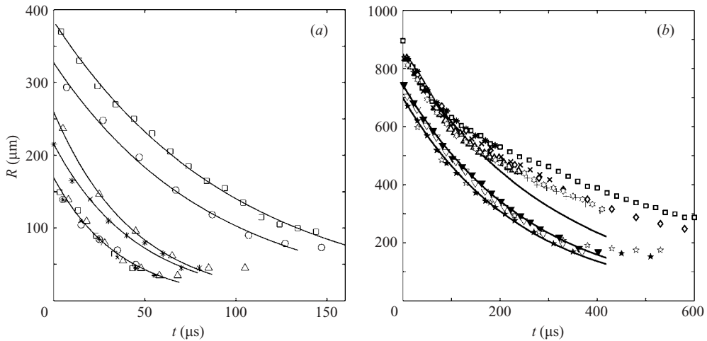
FIGURE 5. The contraction of typical air-disks vs. time, for water drops D = 4.0 mm. (a) From bottom to top the curves are for H = 20.2, 100, 2.25, 5.0 and 9.7 cm. (b) Contraction of the largest air disks, for the three largest R_i in figure 4(a), which occur for slightly different release heights of H = 3.5 ( \star , C = 1.18 ), 3.55 (other symbols, C = 1.35 ) and 3.6 cm ( \nabla , \blacktriangledown , C = 1.02 ).
